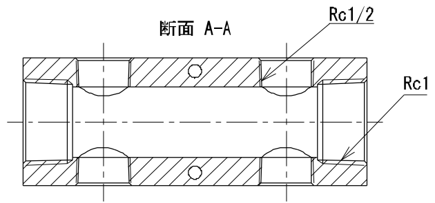
GSH-4PNX-25
